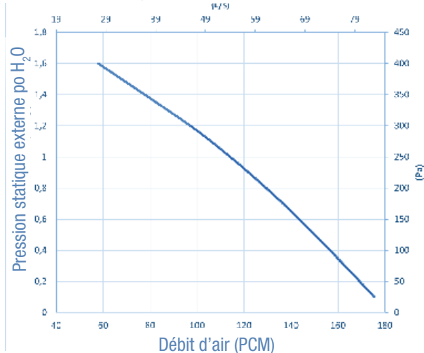
EK150-TQG Performance de ventilation
